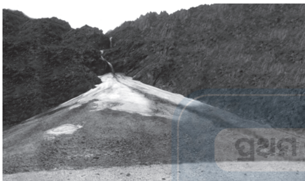
Figure 7.4 : An alluvial fan deposited by a hill stream on the way to Amarnath, Jammu and Kashmir
