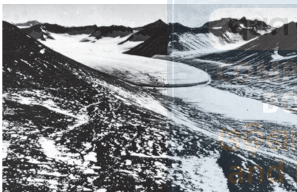
Figure 7.12 : A glacier in its valley
