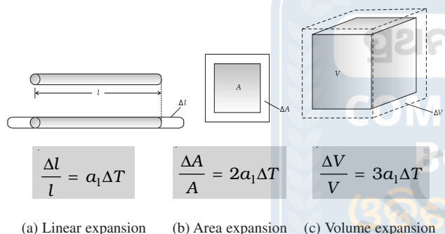
Fig. 11.5 Thermal Expansion.
